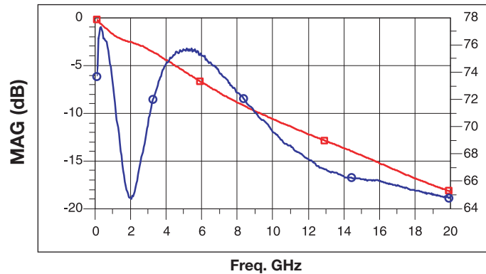
Low Frequency Modeled Loss (S21)
