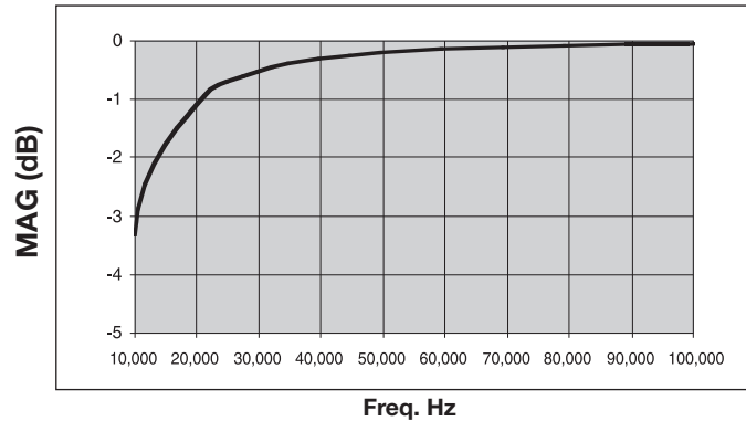
Low Frequency Modeled Loss (S21)
